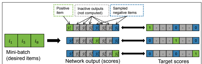
Figure 1: Mini-batch based negative sampling.
